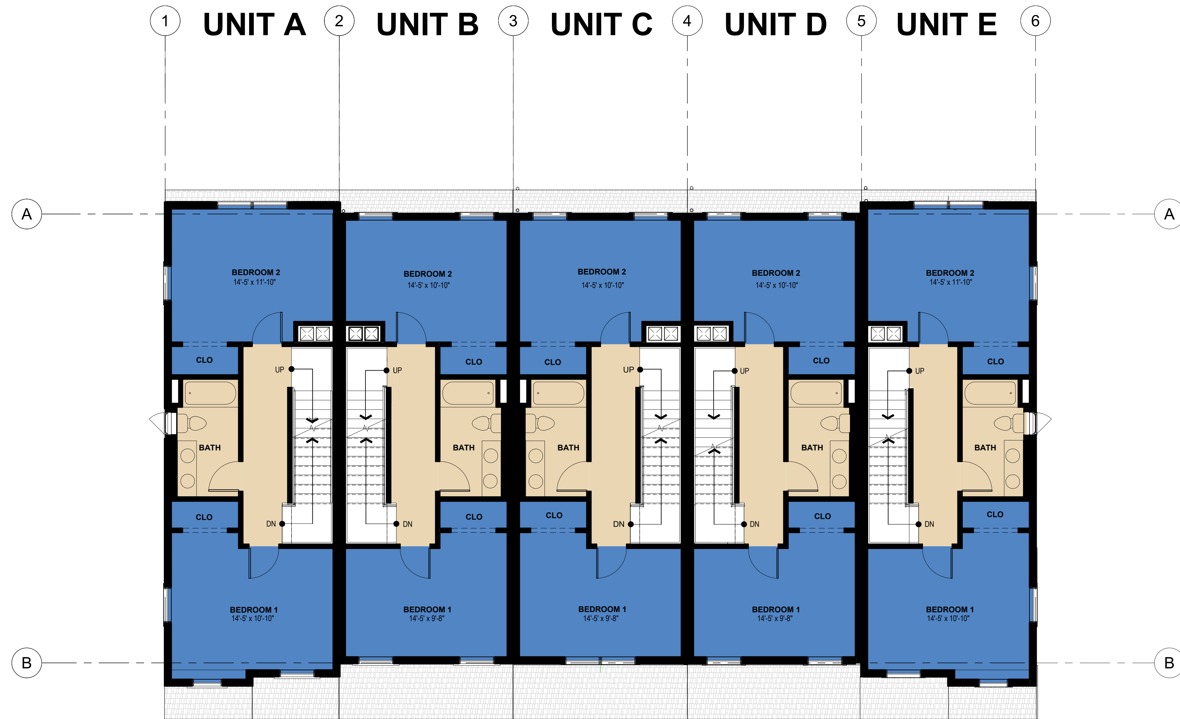
2ND LEVEL
